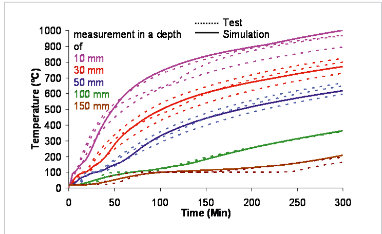
a) Temperature signal – measurement versus simulation (example wall 2)
