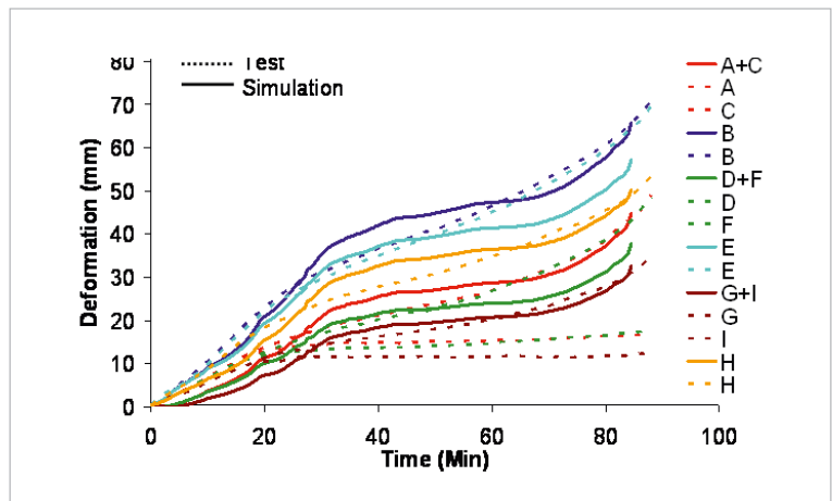
c) Wall 4 (d = 0,15 m) deformation signal – measurement versus simulation
