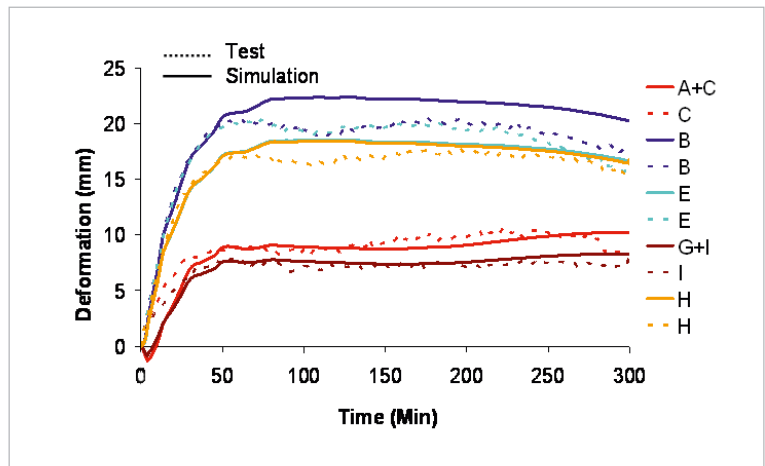
b) Wall 3 (d = 0,214 m) deformation signal – measurement versus simulation
