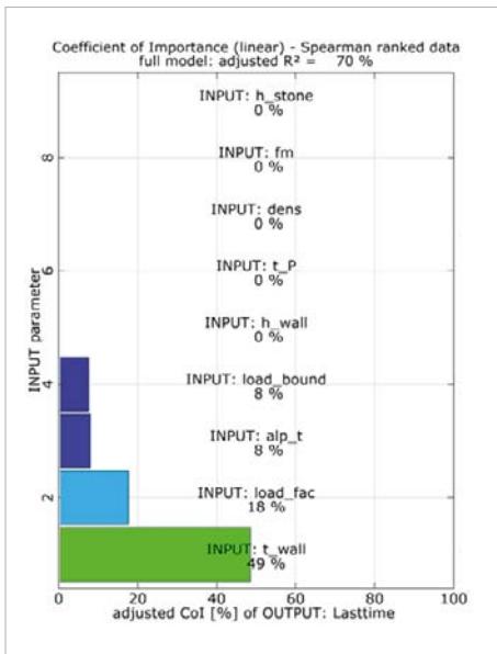
Coefficient of importance of all input parameter versus fire resistance time (walls without plaster)
