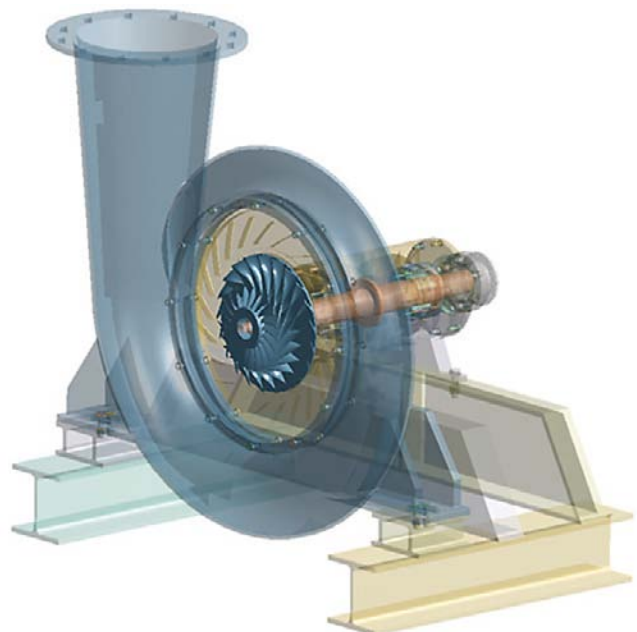
single-stage turbo compressor
